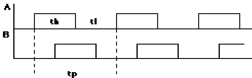
TTL Signal form
